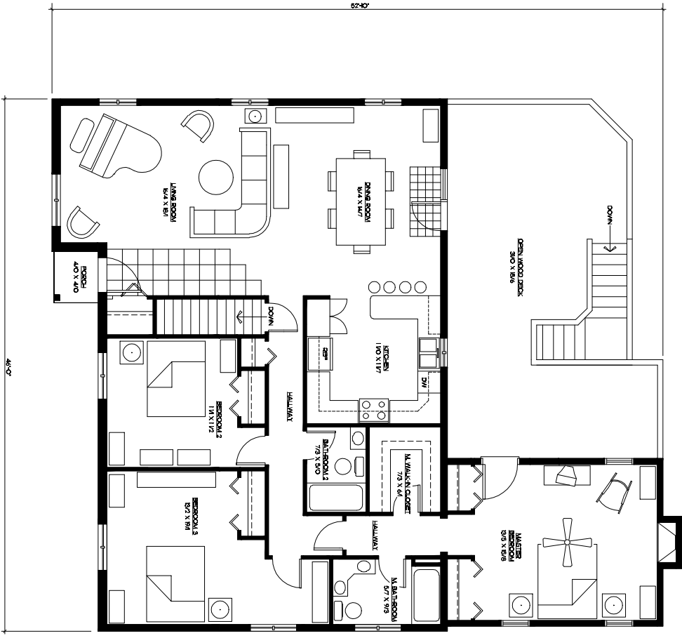
FIRST FLOOR PLAN 1770 SQUARE FEET 1/4"=1'-0"
